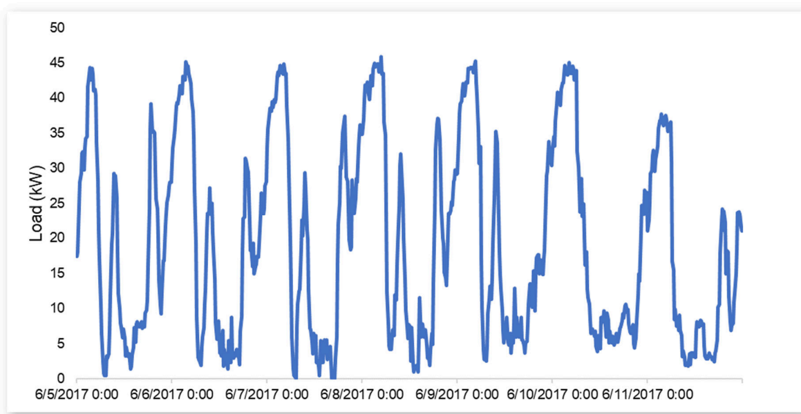
Figure 14. Transit Bus Unmanaged Charging Load (Summer Week)
