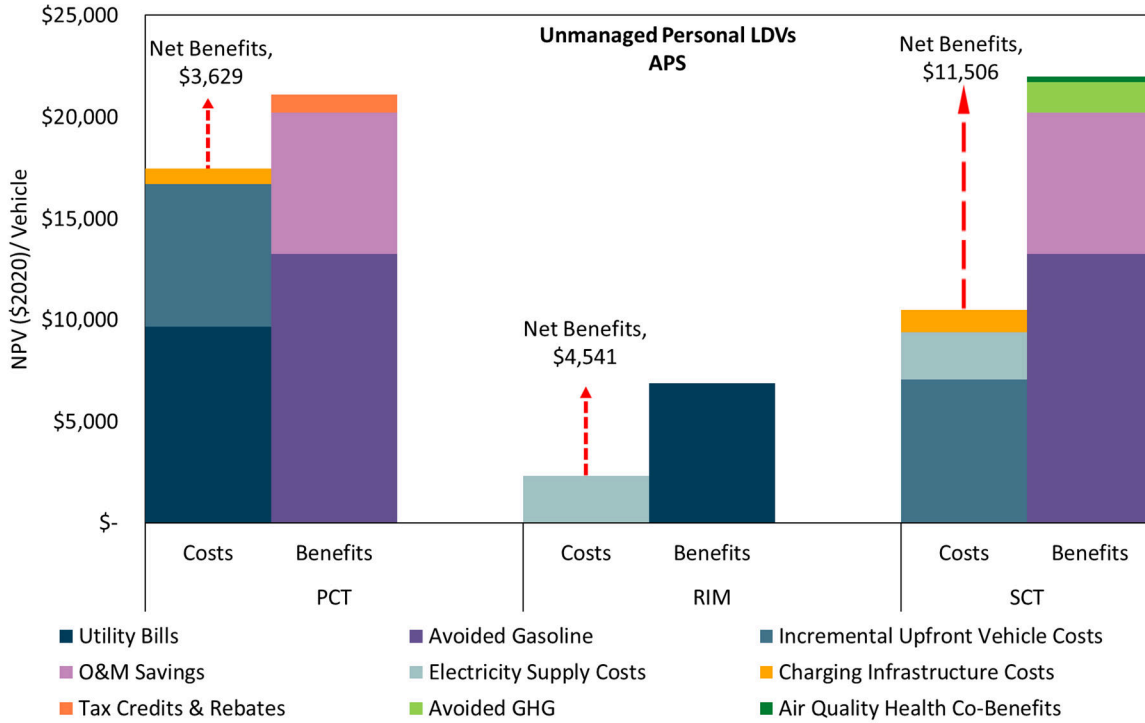
Figure 42. APS Personal LDV Unmanaged
